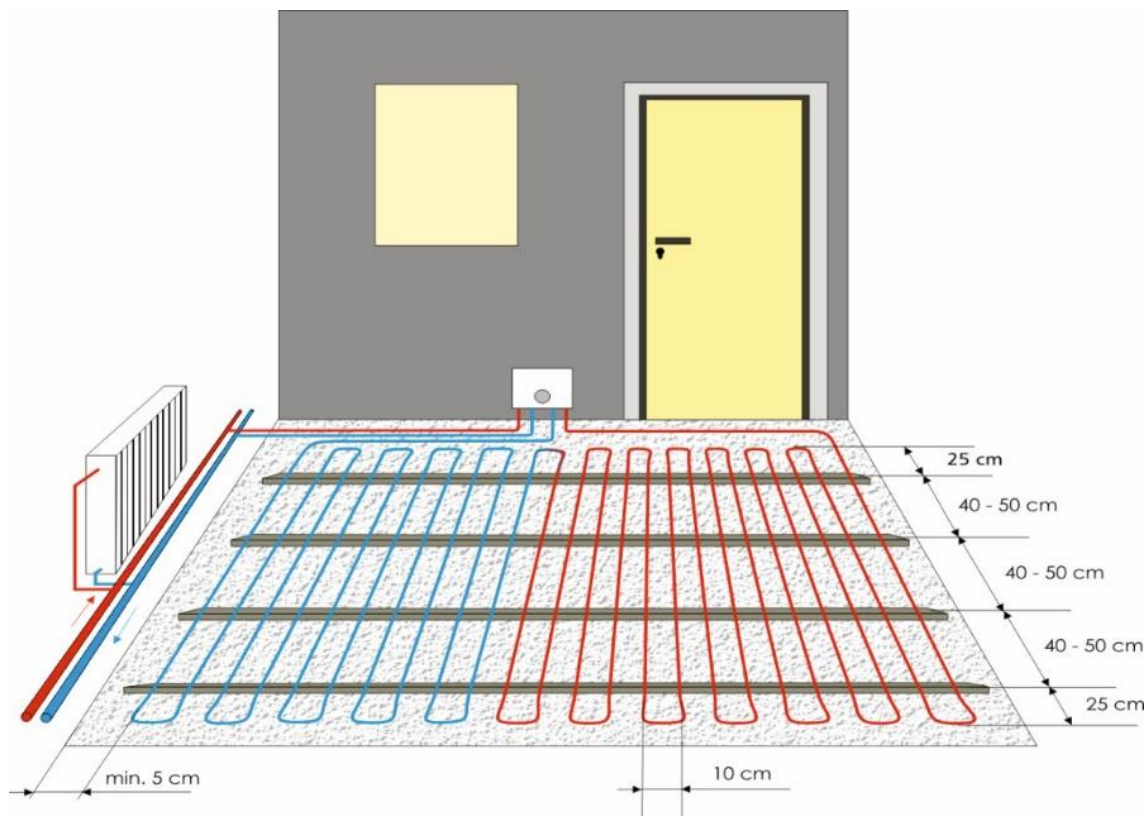
FLEXIRO thin-bed underfloor heating, pipe installation pattern: meandering pattern.
