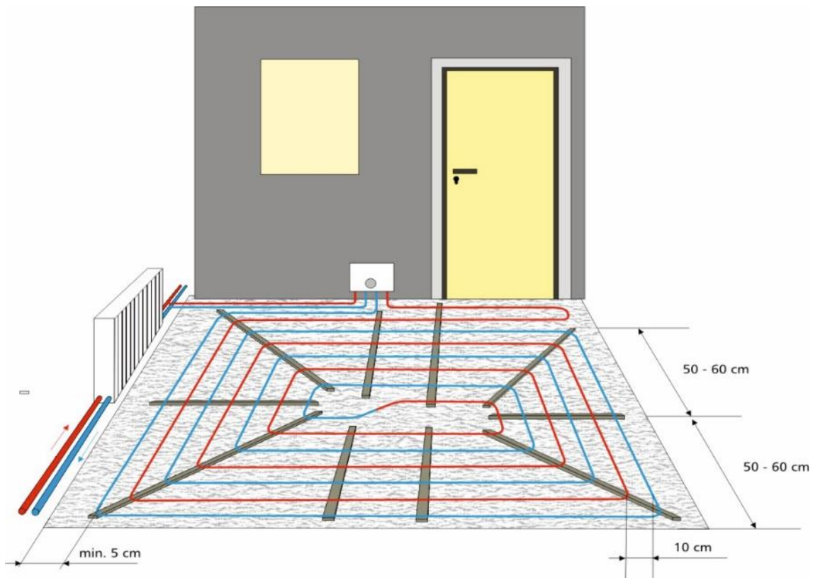
FLEXIRO thin-bed underfloor heating, pipe installation pattern: spiral
